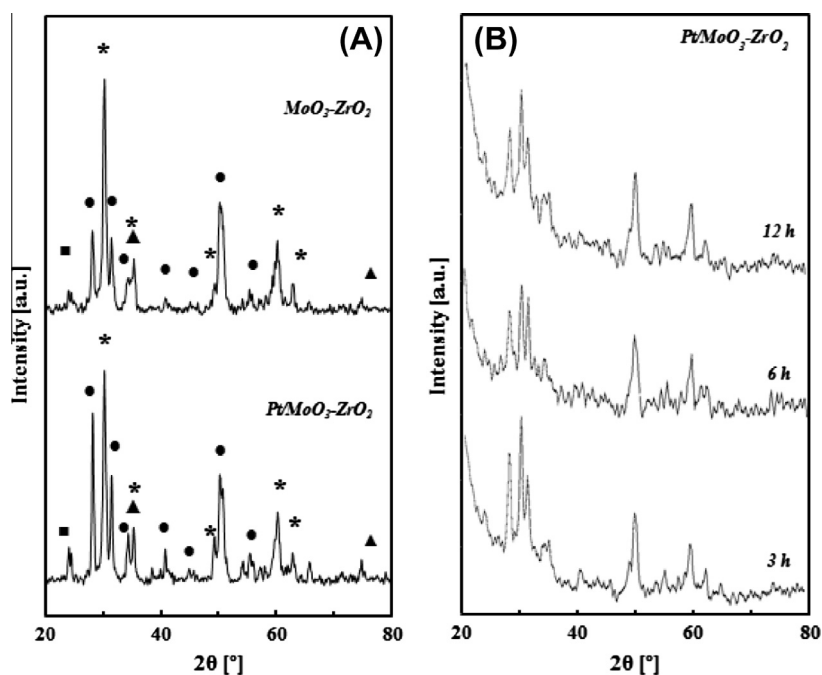
Fig. 1. (A) X-ray diffraction patterns of \text{MoO}_3\text{-ZrO}_2 and \text{Pt}/\text{MoO}_3\text{-ZrO}_2 . (●) Monoclinic phase of \text{ZrO}_2 ; (*) tetragonal phase of \text{ZrO}_2 ; (▲) cubic phase of \text{ZrO}_2 ; (■) \text{Zr}(\text{MoO}_4)_2 phase. (B) X-ray diffraction patterns of \text{Pt}/\text{MoO}_3\text{-ZrO}_2 reduced with \text{H}_2 at 673 K for 3, 6 and 12 h.
