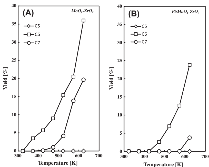
Fig. 9. Yield of isomer products for hydroisomerization of n -pentane, n -hexane and n -heptane at different reaction temperatures over (A) \text{MoO}_3\text{-ZrO}_2 and (B) \text{Pt/MoO}_3\text{-ZrO}_2 .
