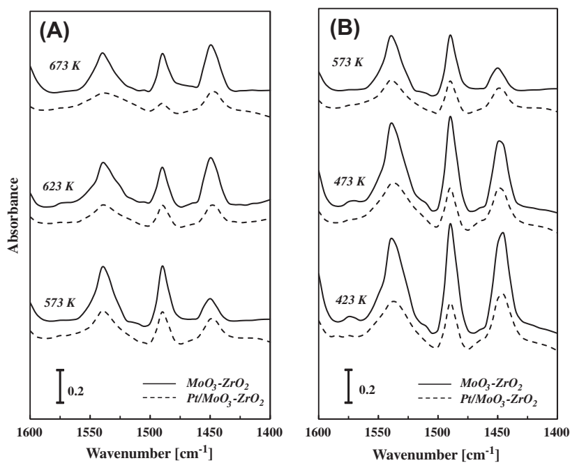
Fig. 3. (A) IR spectra of pyridine adsorbed on MoO_3-ZrO_2 and Pt/MoO_3-ZrO_2 samples activated at different temperatures. Pyridine was adsorbed at 423 K and outgassed at 573 K. (B) IR spectra of pyridine adsorbed on MoO_3-ZrO_2 and Pt/MoO_3-ZrO_2 at 423 K and outgassed at different temperatures. Samples were activated at 573 K.
