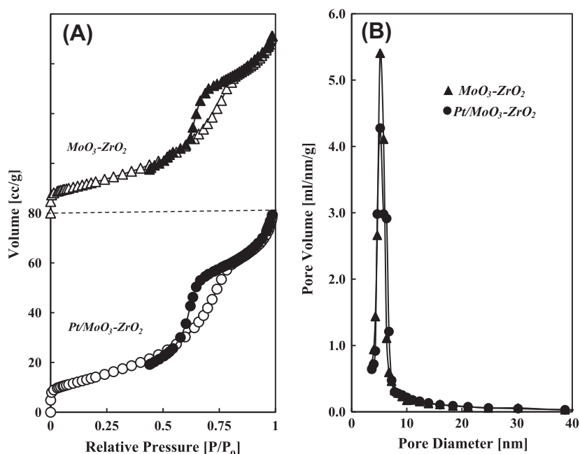
Fig. 2. (A) Adsorption–desorption isotherms of N_2 on MoO_3-ZrO_2 and Pt/MoO_3-ZrO_2 . Open and solid symbols represent adsorption and desorption isotherms, respectively. (B) Pore size distribution of MoO_3-ZrO_2 and Pt/MoO_3-ZrO_2 .
