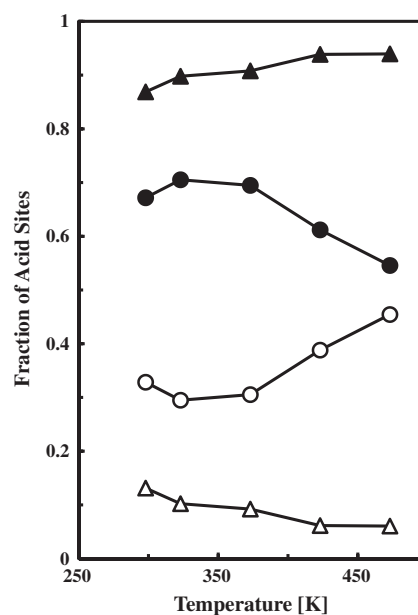
Fig. 6. Plot of ( \blacktriangle, \triangle ) \text{MoO}_3\text{-ZrO}_2 and ( \bullet, \circ ) \text{Pt/MoO}_3\text{-ZrO}_2 pre-adsorbed pyridine followed by heating in the presence of hydrogen. Solid symbol: Brønsted acid sites; open symbol: Lewis acid sites.
