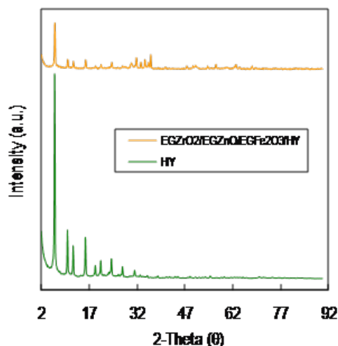
Fig. 1. XRD patterns of photocatalysts for full range 2–92°.
