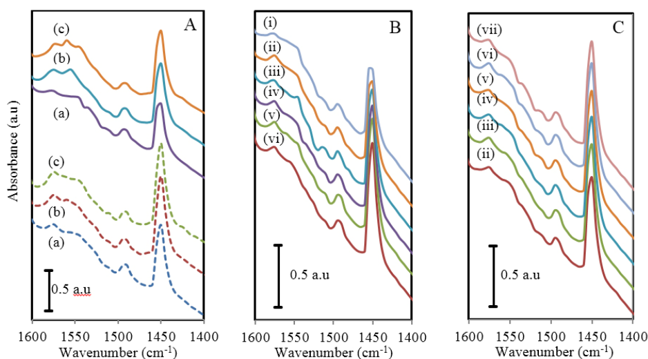
Fig. 5 (A) Pyridine adsorbed IR spectra of (a) 1.0 ZnO/MoO 3 -ZrO 2 , 2.5 ZnO/MoO 3 -ZrO 2 and 5.0 ZnO/MoO 3 -ZrO 2 at treatment of 523 K (dashed lines) and 573 K (solid lines), Hydrogen (B) adsorption and (C) desorption spectra of 2.5 ZnO/MoO 3 -ZrO 2 at (i) 298 K, (ii) 298 K, (iii) 323 K, (iv) 423 K, (v) 473 K, (vi) 523 K and (vii) 573 K
