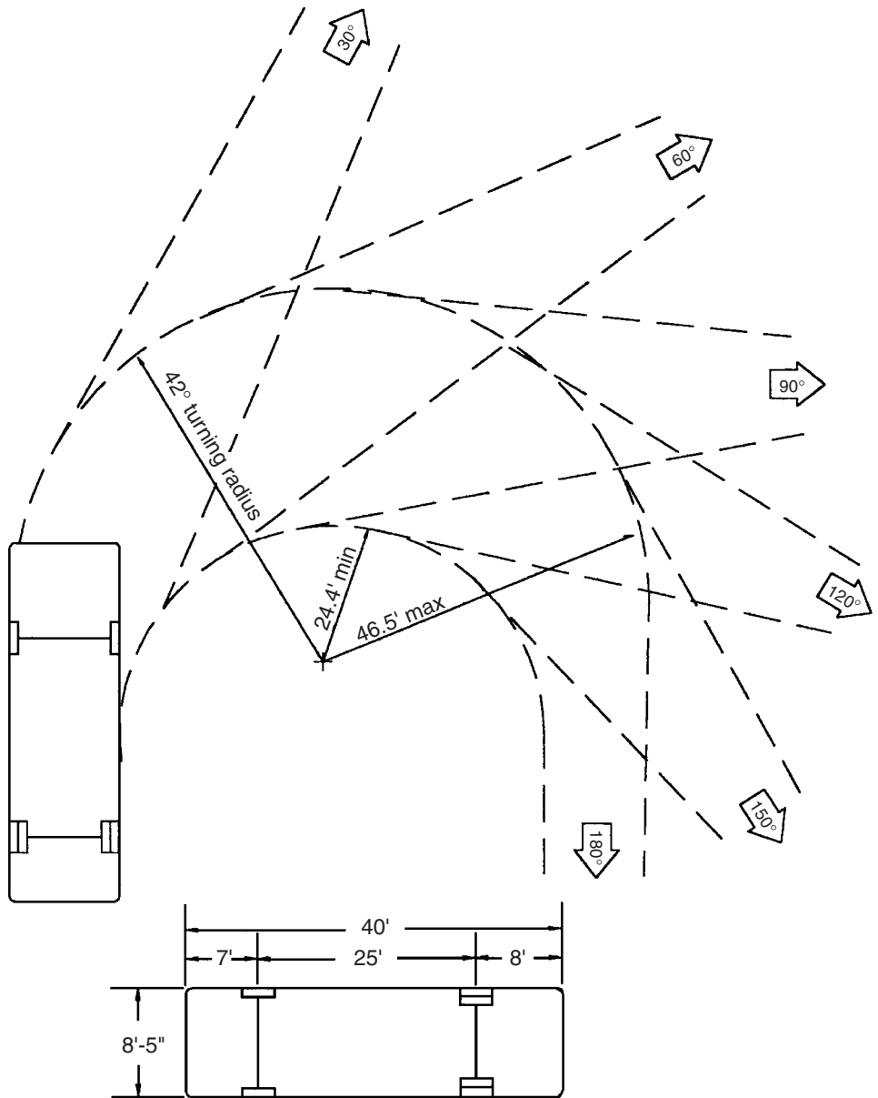
Figure 5.9 Minimum turning path for single unit bus detail. (Copyright © 1994 by the American Association of State Highway and Transportation Officials, Washington, D.C. Used with Permission.)
