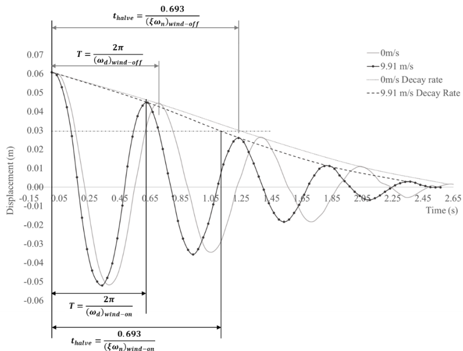
Figure 4: Time response graph of CAMAR-3 with V-tail at 0 m/s and 9.91 m/s wind tunnel test.
