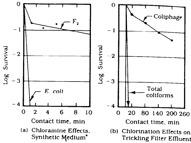
Figure 17.4. Chloramine Effects on Bacteria and Virus
