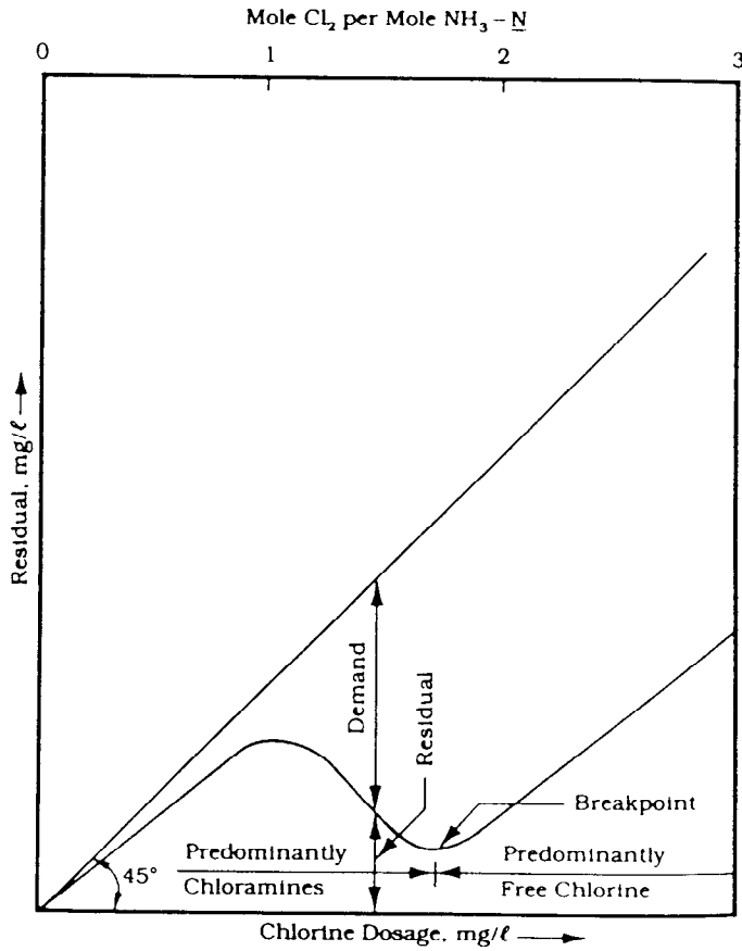
Figure 17.5. Chlorine Dosages, Demands, and Residuals
