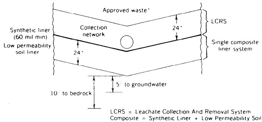
Figure 5-20 Industrial/commercial and ash monofill waste landfills. (Source: New York State Dept of Environmental Conservation, Division of Solid Waste, Albany, N.Y., 1990, 6 NYCRR Part 360 2.14.)
