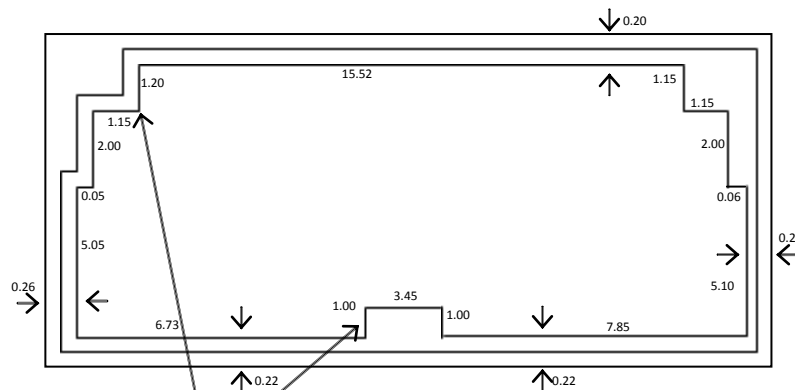
GAMBAR RAJAH 'C'
