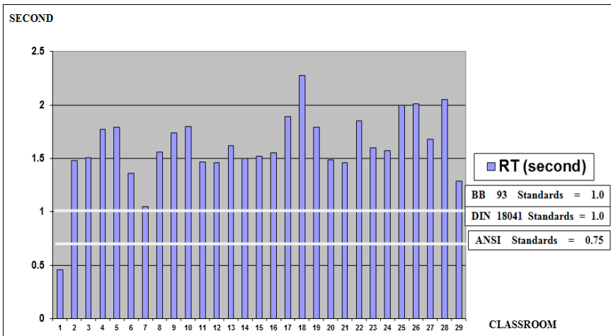
Figure 5.5 Comparison of RT for classrooms with International Standard for the octave band of 2000Hz
