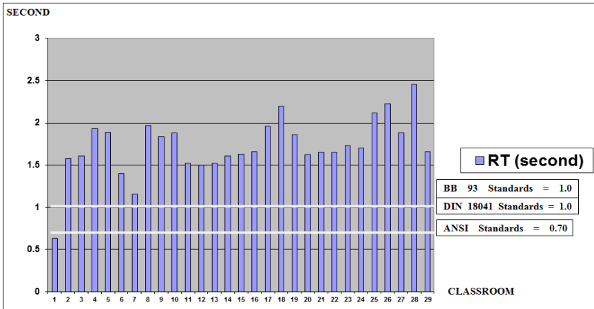
Figure 5.4 Comparison of RT for classrooms with International Standard for the octave band of 1000Hz
