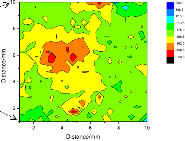
SKP potential map
