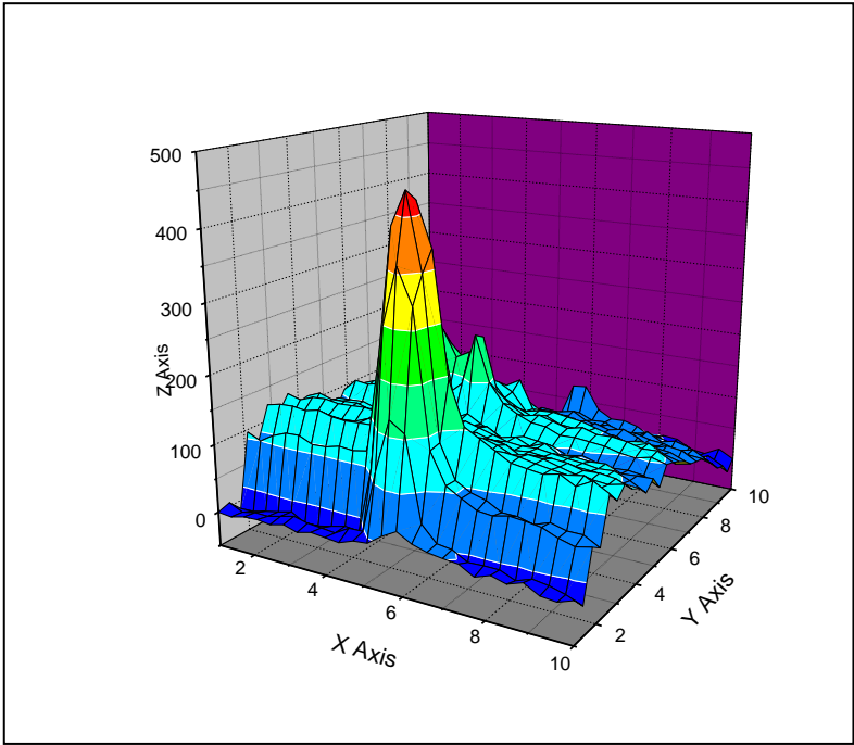
SKP topography map on blister area
